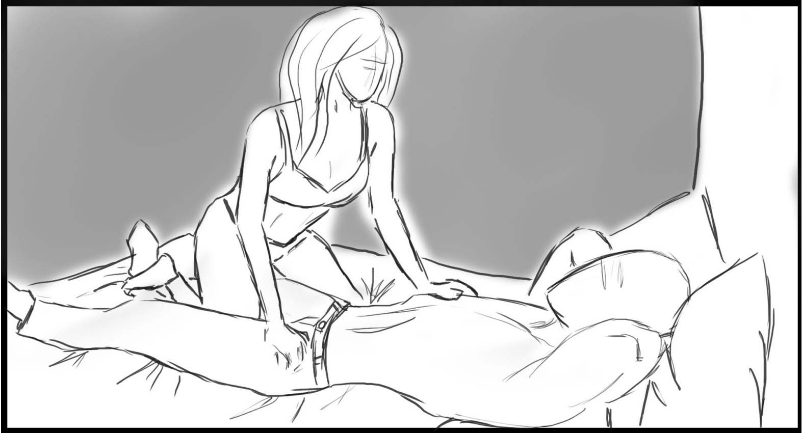
Scene: 60.1
