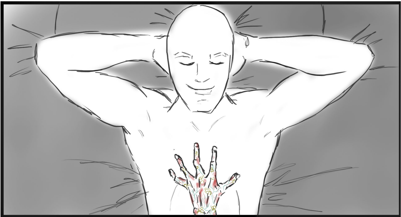
Scene: 60.2
